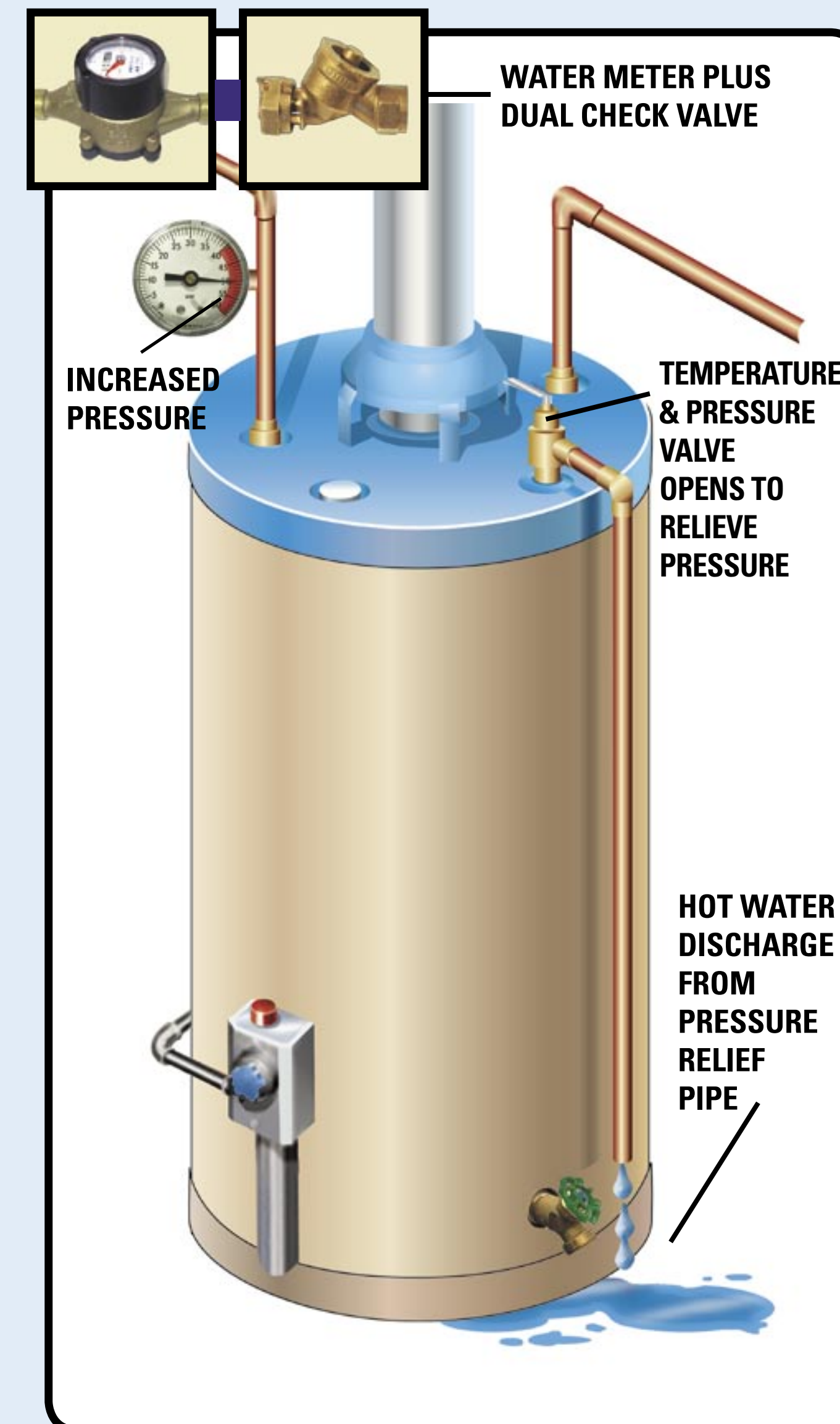
DUAL CHECK VALVE INSTALLED AT METER
